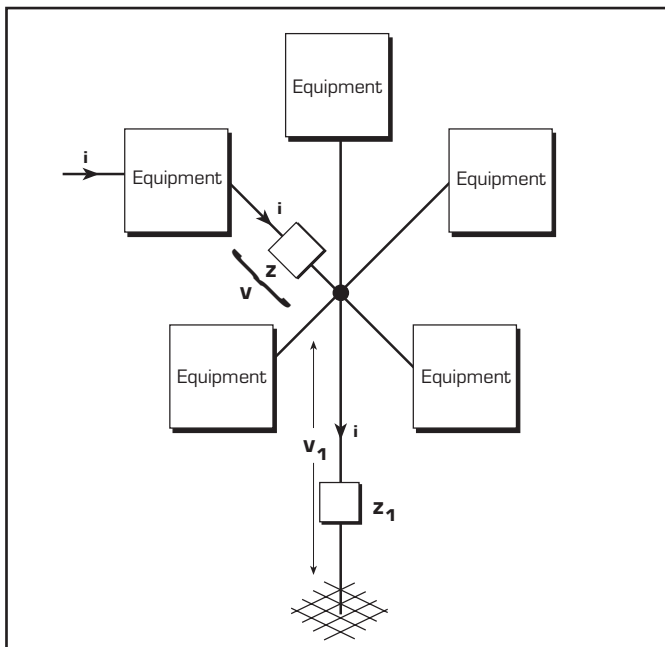
Figure 23 Current flow through one device in a star-point earth system
