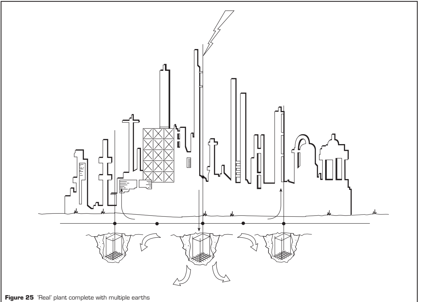
Figure 24 'Ideal' plant with a single earth
